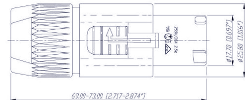
NAC3FCA (20A)
