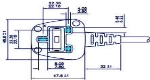
Plug Fuse: 3A
