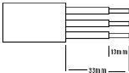
Cable Stripping Details.
