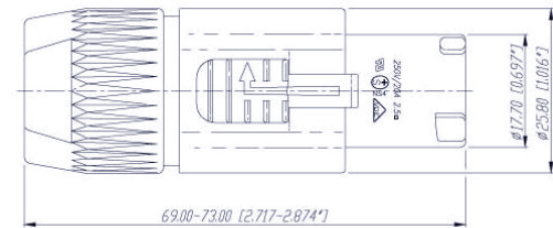
NAC3FCA (20A)
